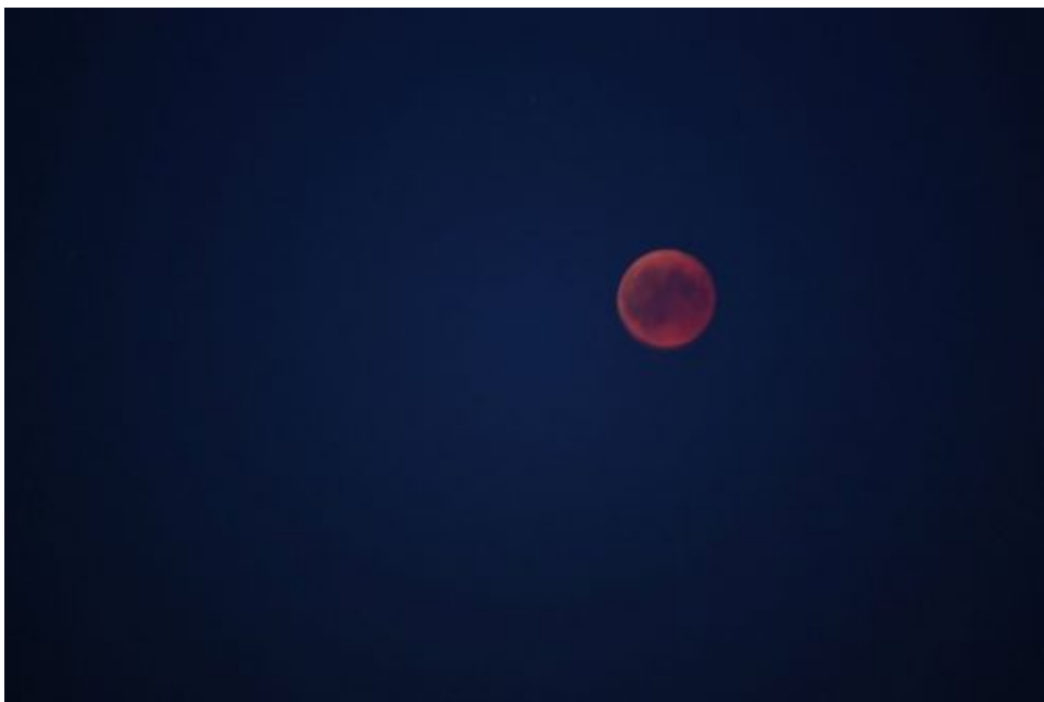
Mondfinsternis 2018
