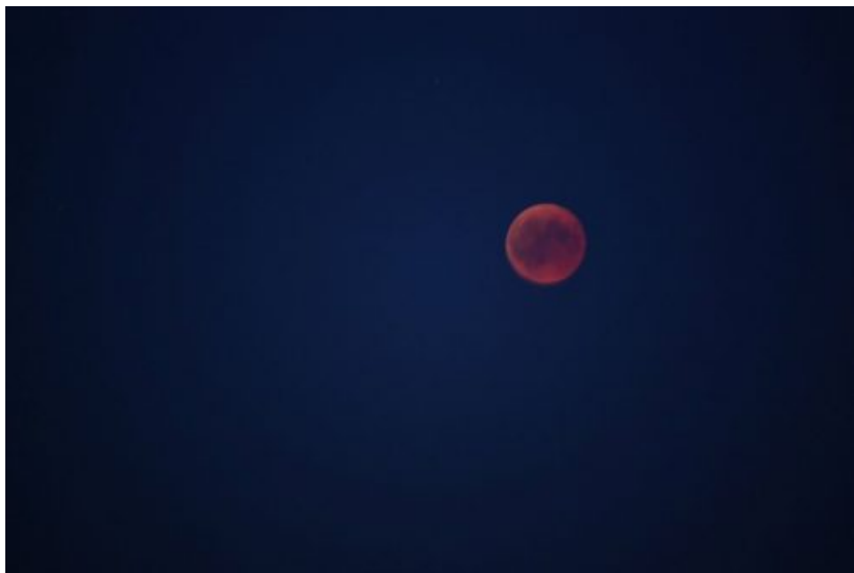
Mondfinsternis 2018
